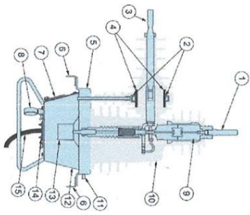
Cross section of PMSet U-Series
